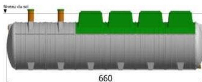
Tricel Seta Simplex FR9/6000
