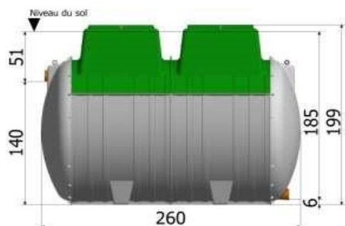
Tricel Seta Simplex FR4/1800
